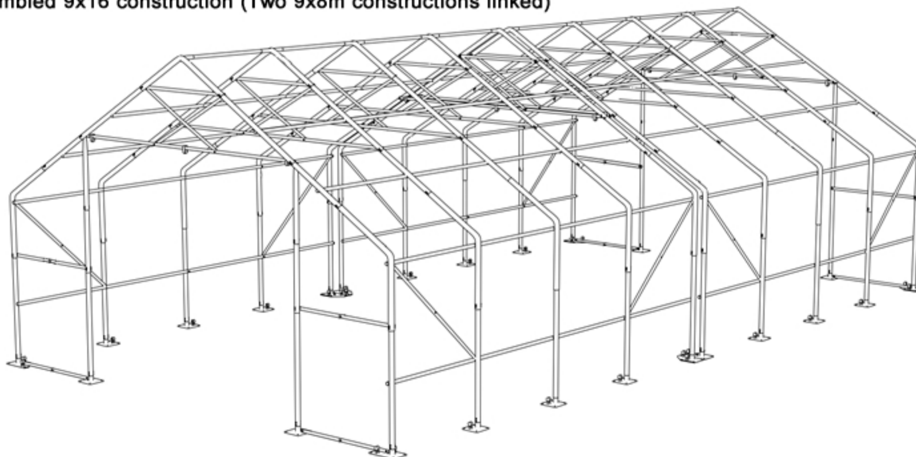
Assembled 9x16 construction (Two 9x8m constructions linked)
